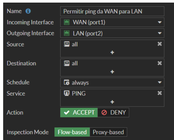
Figura 4.12: Firewall policy in FortiGate allowing ICMP from the WAN network to the LAN.
